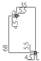
Screw mounting
