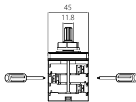
Wiring diagram
